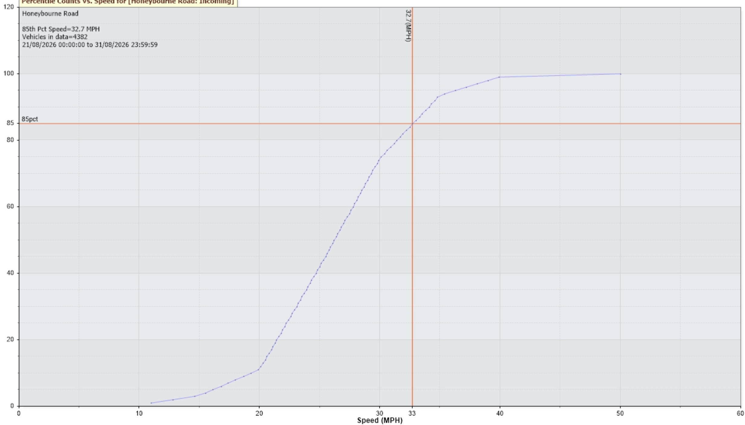
Percentile Counts Vs. Speed for [Honeybourne Road: Incoming]
