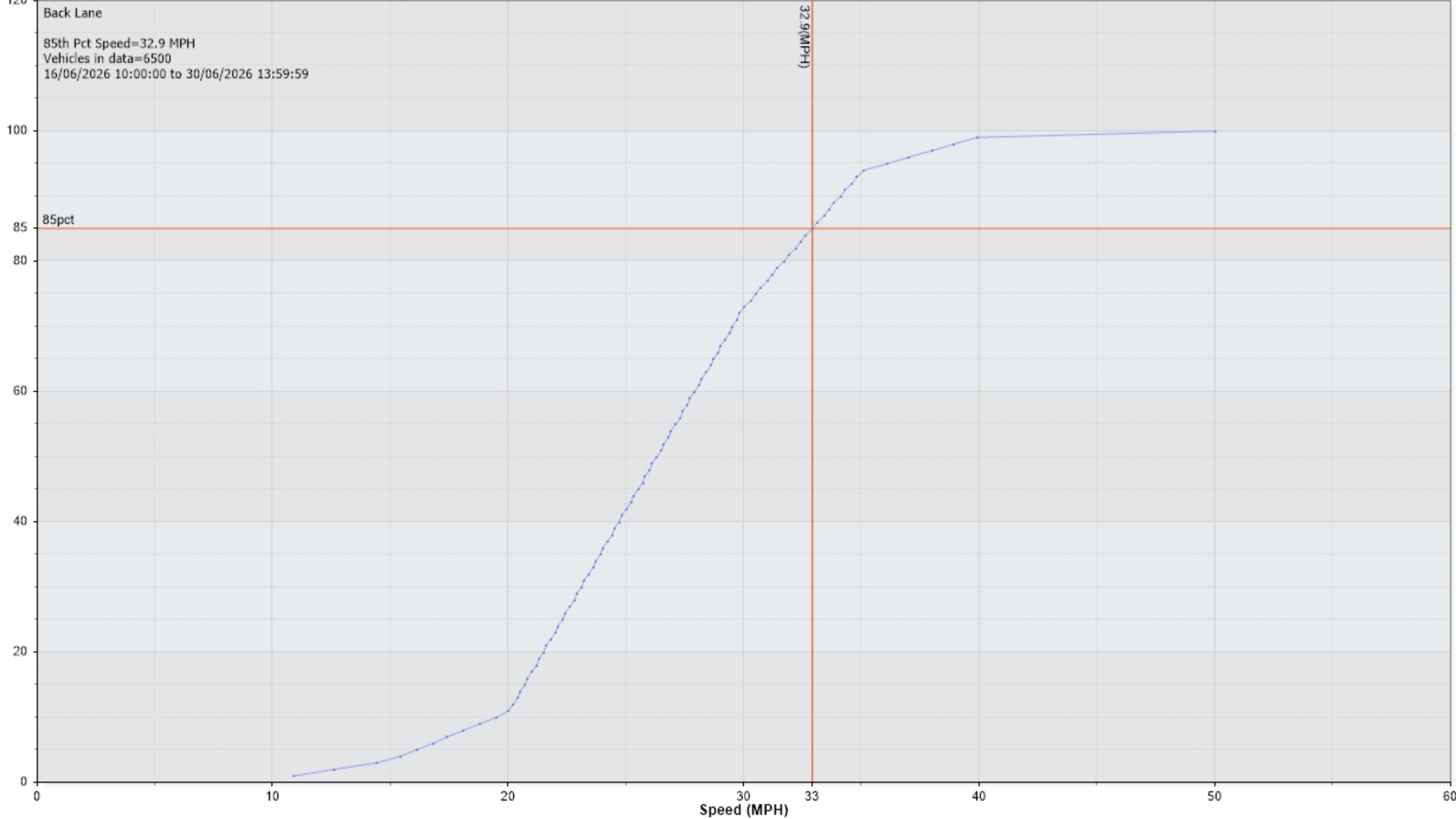
Percentile Counts Vs. Speed for [Back Lane: Incoming]
