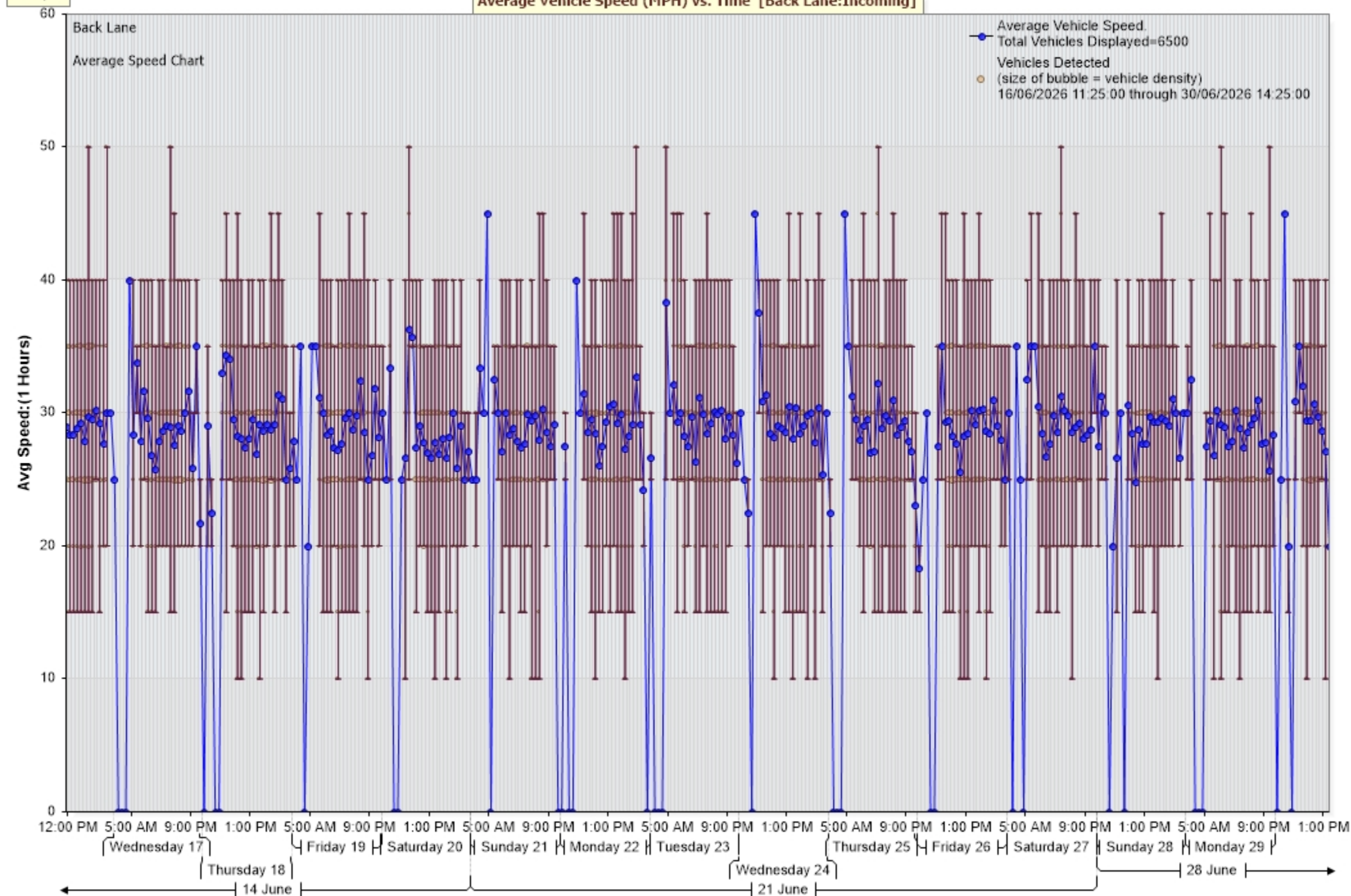
Average Vehicle Speed (MPH) vs. Time [Back Lane:Incoming]
