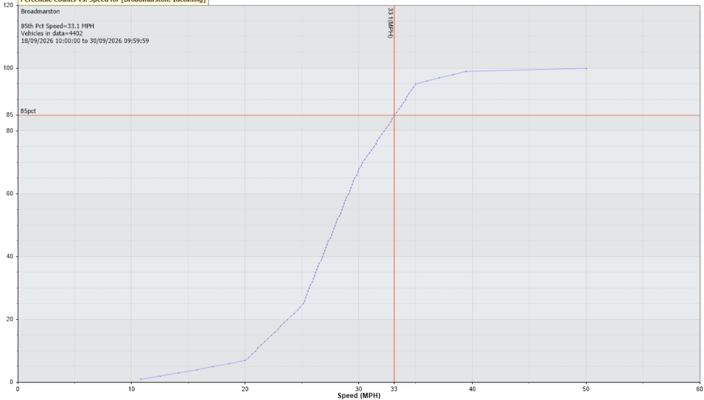
Percentile Counts Vs. Speed for [Broadmarston: Incoming]
