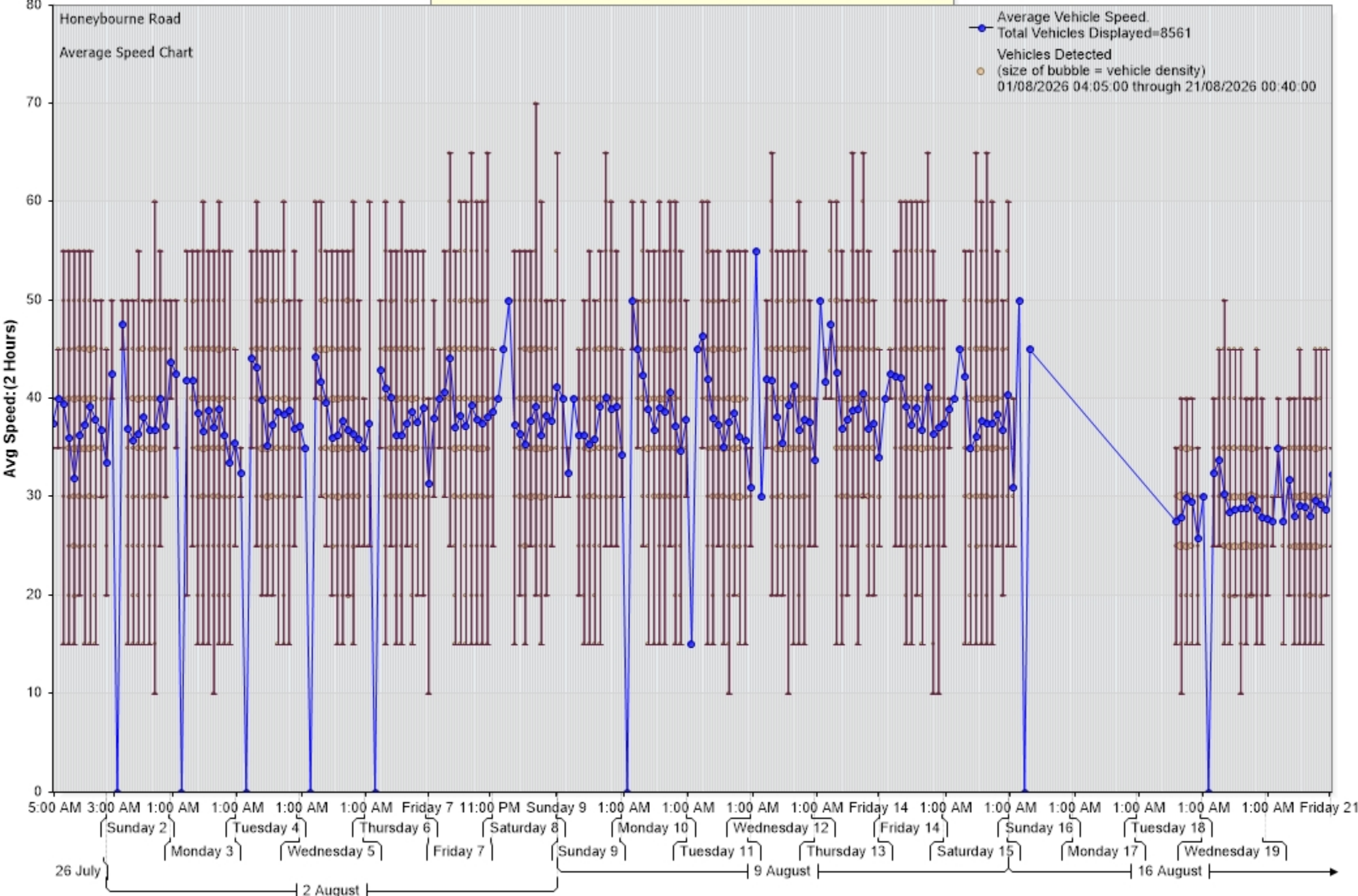
Average Vehicle Speed (MPH) vs. Time [Honeybourne Road:Incoming]
