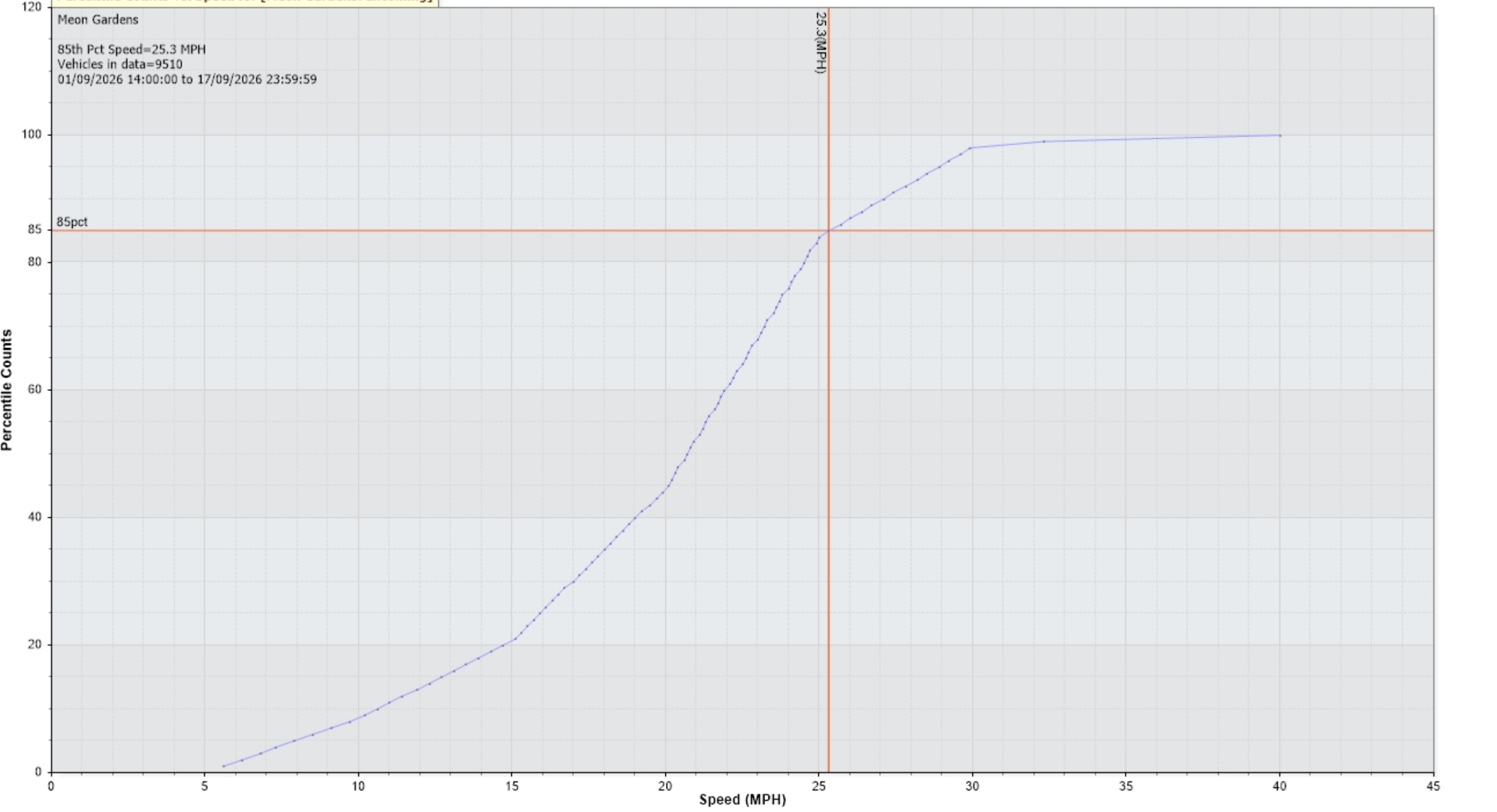
Percentile Counts Vs. Speed for [Meon Gardens: Incoming]
